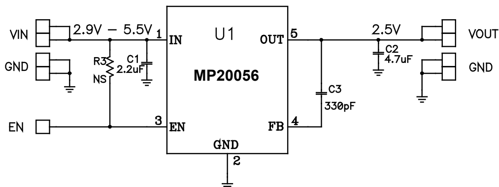
Figure 5: 2.5V Fixed Output Application (TSOT23-5L)
