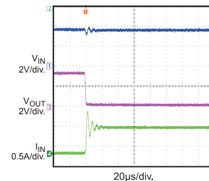
Short Output
